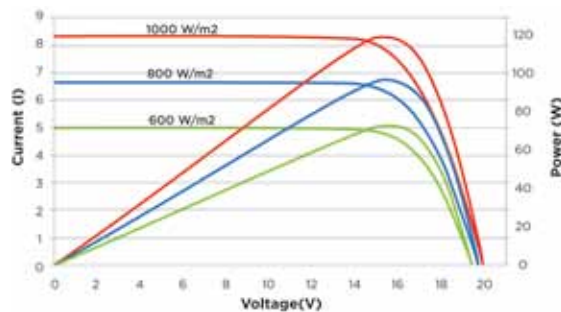
RI 6 (32) Characteristics IV/Power Curves against Incident Radiation (at 25°C)
