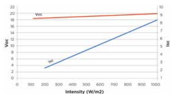
RI 6 (32) Characteristics Curves: Isc, Voc vs Radiation Intensity
